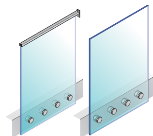
Visible Screw Fix Type 316 Stainless Steel Satin Finish 75mm
